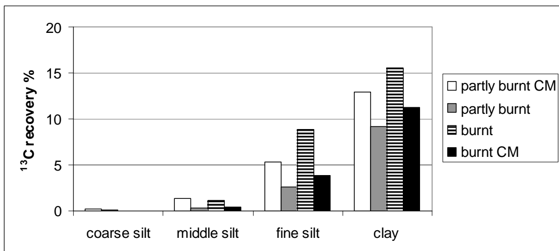
Figure 1. ^{13}\text{C} Recovery of char of the particle size fractions after 6 months of incubation (CM means addition of fresh plant material)
